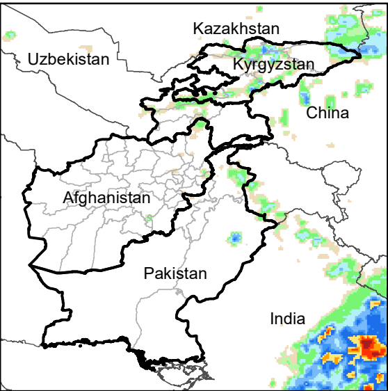
Daily Rainfall estimate for 13 Oct., 2022
