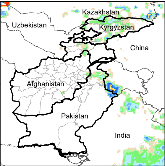
Daily Rainfall estimate for 14 Oct., 2022
