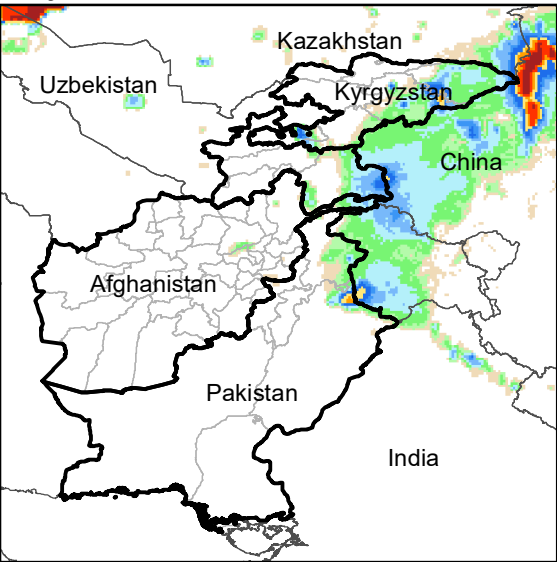
Daily Rainfall estimate for 23 Oct., 2022
