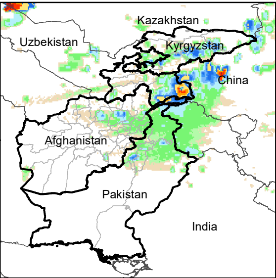
Daily Rainfall estimate for 16 Nov., 2022
