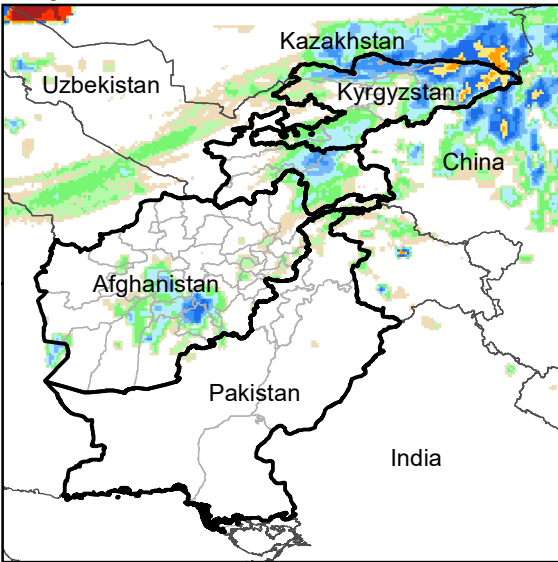
Daily Rainfall estimate for 7 Dec., 2022
