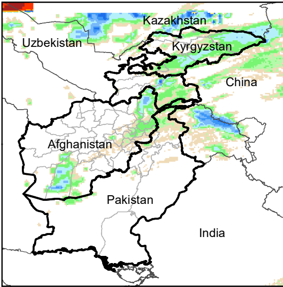
Daily Rainfall estimate for 8 Dec., 2022
