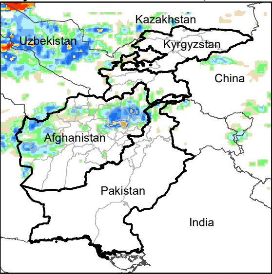
Daily Rainfall estimate for 15 Dec., 2022
