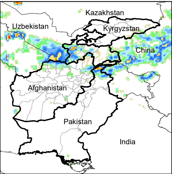
Daily Rainfall estimate for 22 Dec., 2022
