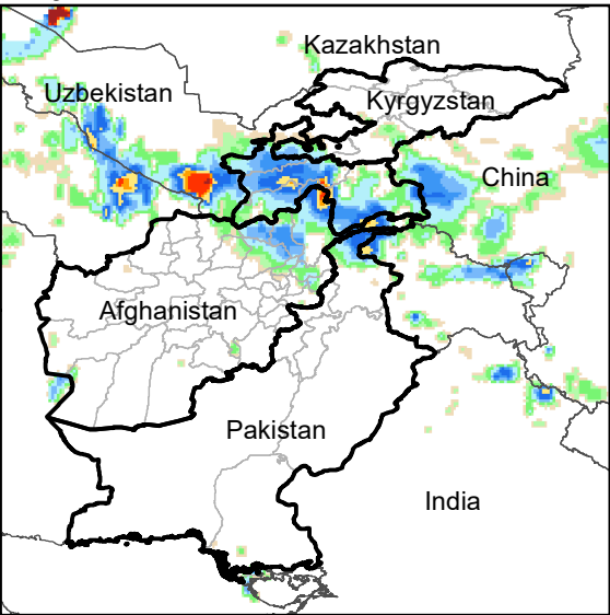
Daily Rainfall estimate for 23 Dec., 2022
