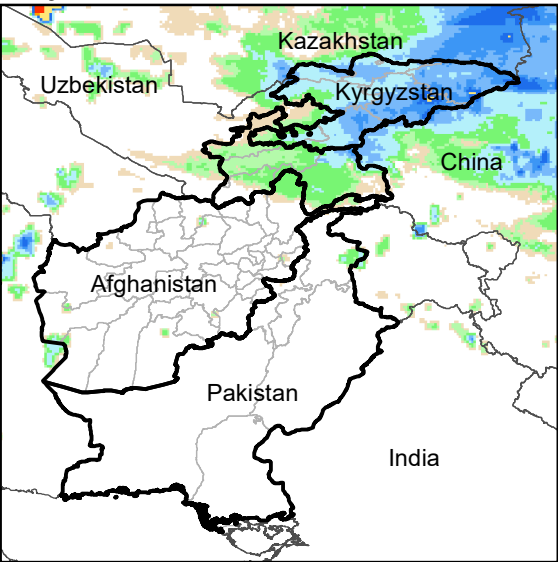
Daily Rainfall estimate for 7 Jan., 2023
