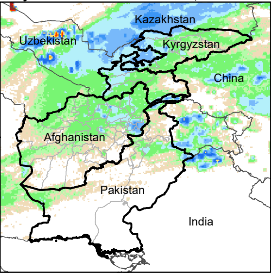
Daily Rainfall estimate for 6 Jan., 2023
