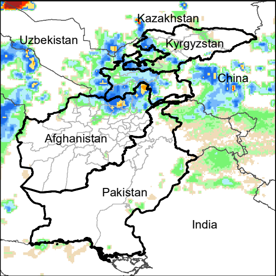
Daily Rainfall estimate for 19 Jan., 2023
