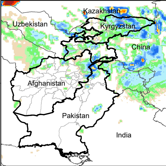
Daily Rainfall estimate for 20 Jan., 2023
