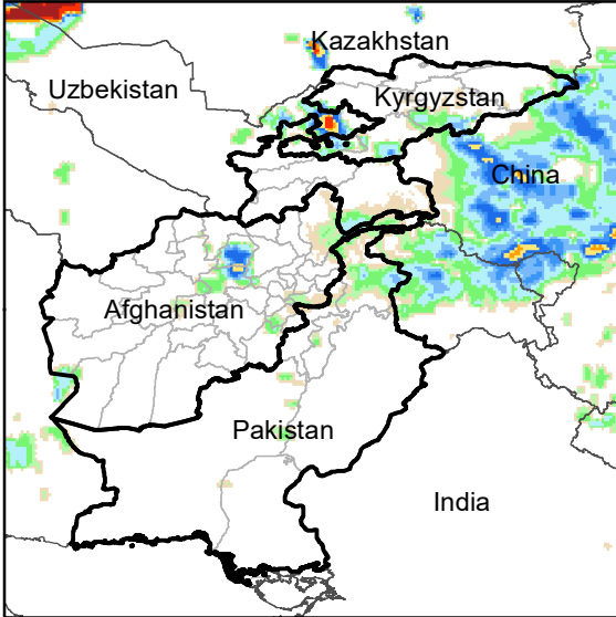
Daily Rainfall estimate for 21 Jan., 2023
