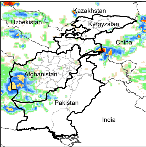
Daily Rainfall estimate for 17 Jan., 2023
