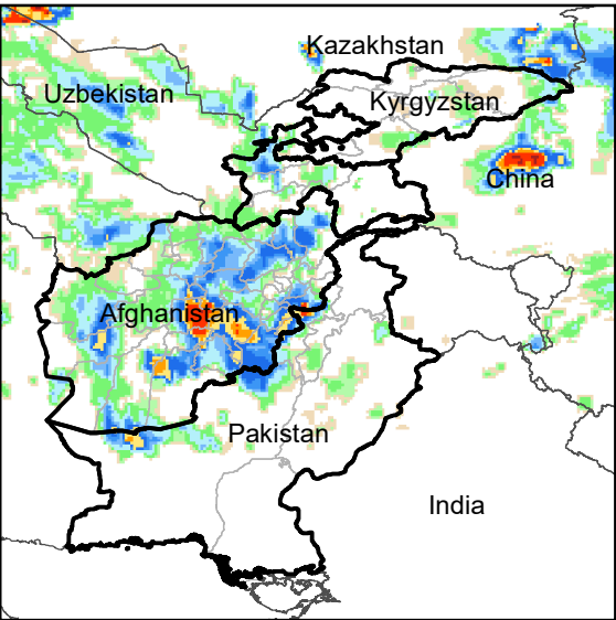
Daily Rainfall estimate for 16 Jan., 2023
