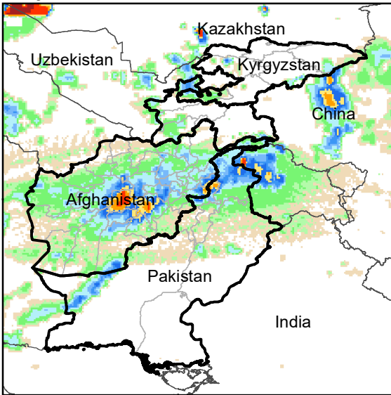
Daily Rainfall estimate for 18 Jan., 2023
