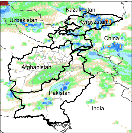
Daily Rainfall estimate for 4 Mar., 2023
