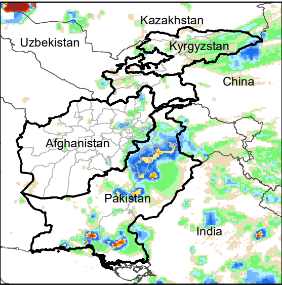
Daily Rainfall estimate for 16 Mar., 2023
