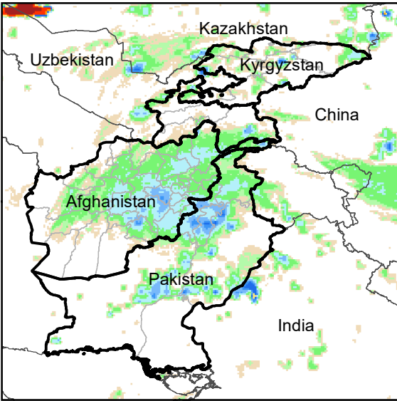
Daily Rainfall estimate for 29 Mar., 2023
