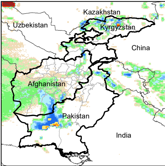
Daily Rainfall estimate for 30 Mar., 2023
