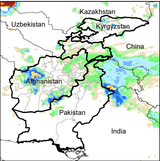
Daily Rainfall estimate for 28 Mar., 2023
