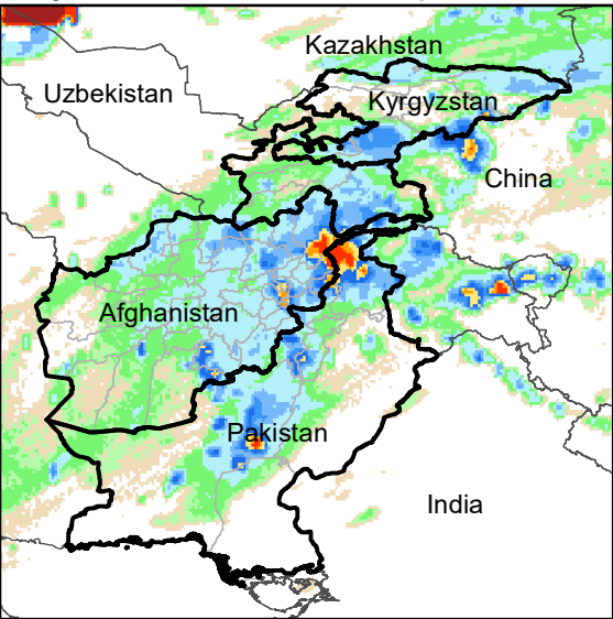
Daily Rainfall estimate for 20 Apr., 2023
