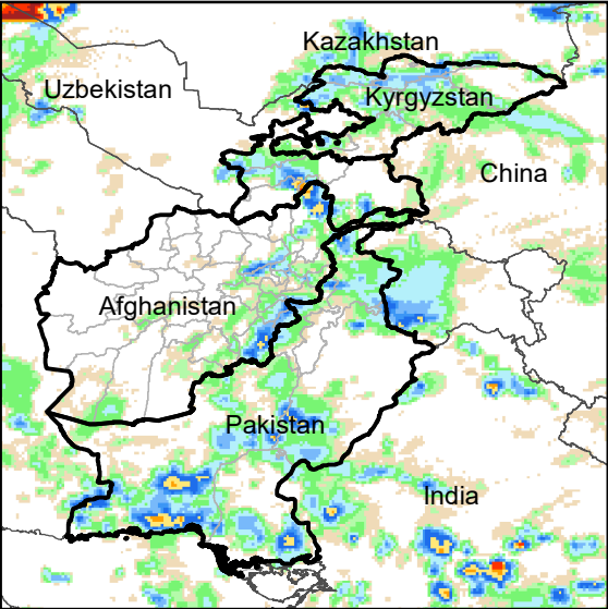
Daily Rainfall estimate for 28 Apr., 2023
