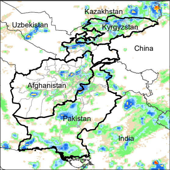
Daily Rainfall estimate for 29 Apr., 2023
