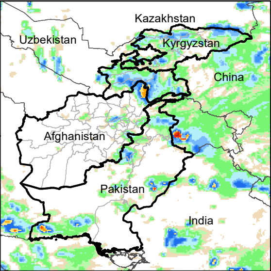
Daily Rainfall estimate for 27 Apr., 2023
