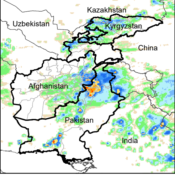
Daily Rainfall estimate for 1 May., 2023
