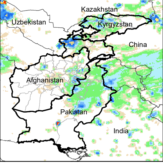
Daily Rainfall estimate for 2 May., 2023
