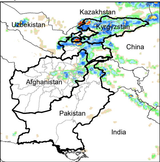
Daily Rainfall estimate for 11 Jun., 2023
