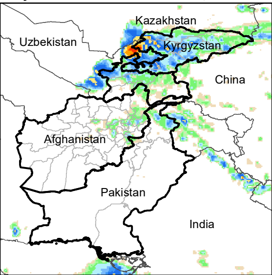
Daily Rainfall estimate for 12 Jun., 2023
