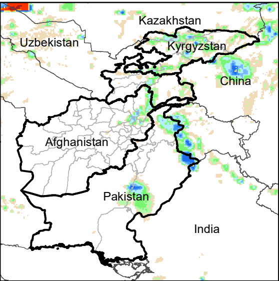
Daily Rainfall estimate for 10 Jun., 2023
