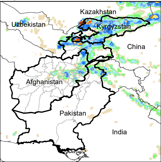
Daily Rainfall estimate for 14 Jun., 2023
