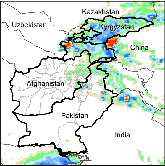
Daily Rainfall estimate for 13 Jun., 2023
