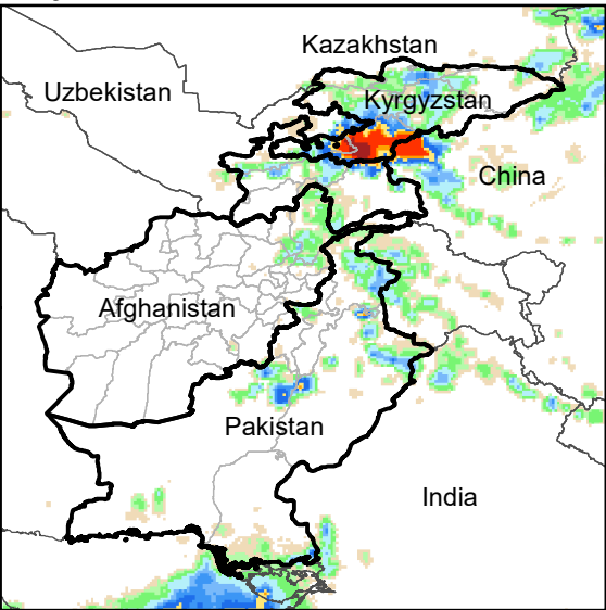
Daily Rainfall estimate for 18 Jun., 2023
