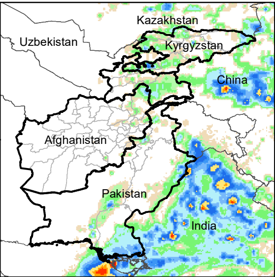
Daily Rainfall estimate for 11 Jul., 2023
