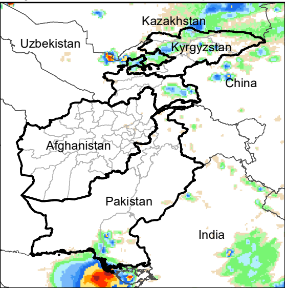
Daily Rainfall estimate for 23 Sep., 2023
