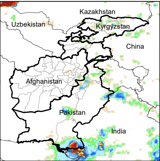
Daily Rainfall estimate for 21 Sep., 2023
