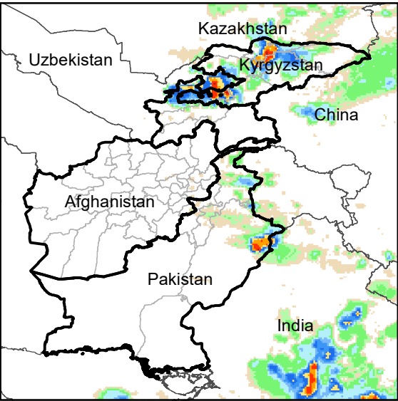
Daily Rainfall estimate for 22 Sep., 2023
