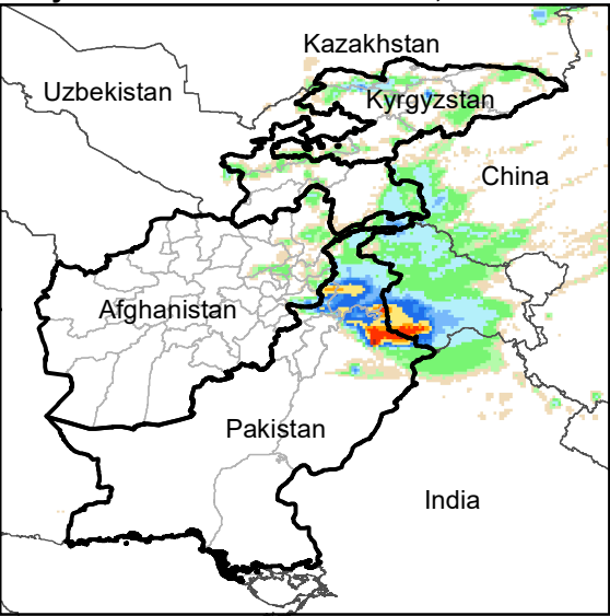
Daily Rainfall estimate for 9 Oct., 2023
