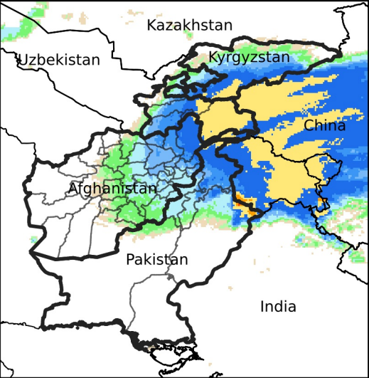
Daily Rainfall estimate for Feb 22, 2024
