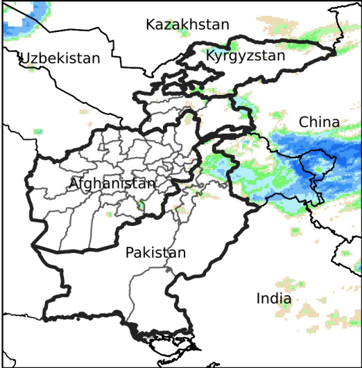
Daily Rainfall estimate for Feb 24, 2024
