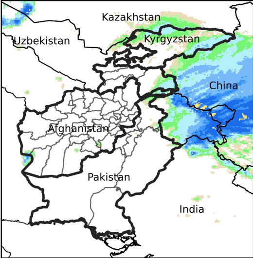
Daily Rainfall estimate for Feb 23, 2024
