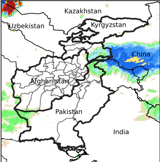
Daily Rainfall estimate for Mar 4, 2024
