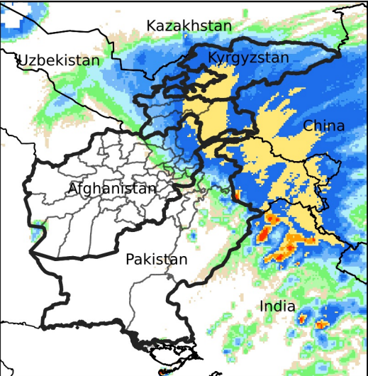
Daily Rainfall estimate for Mar 2, 2024
