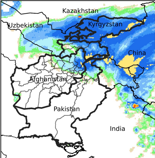
Daily Rainfall estimate for Mar 3, 2024
