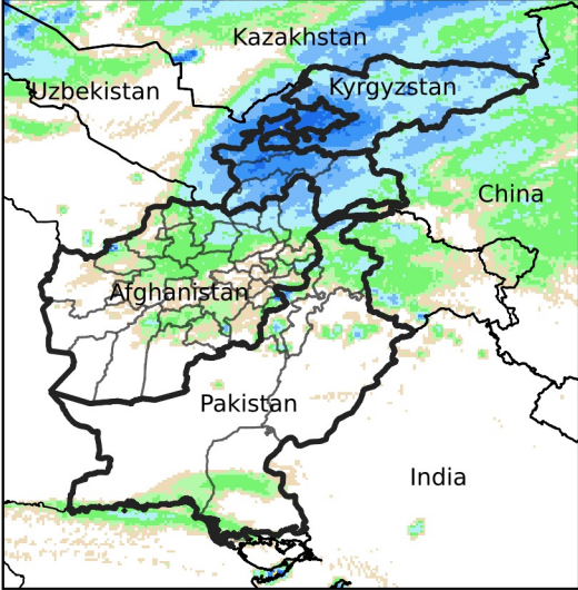
Daily Rainfall estimate for Mar 21, 2024
