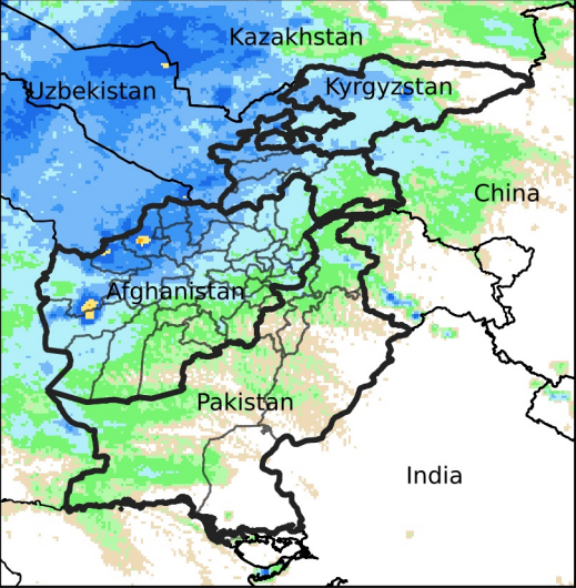
Daily Rainfall estimate for Mar 20, 2024
