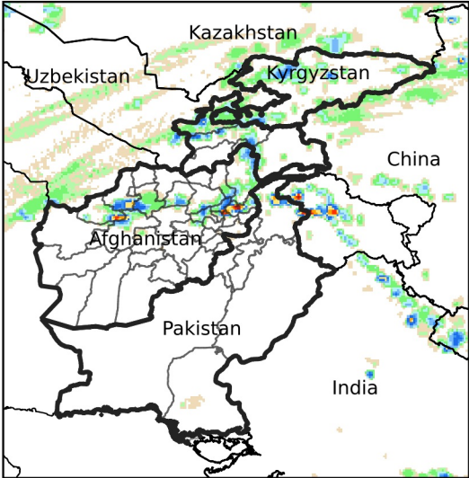
Daily Rainfall estimate for May 25, 2024
