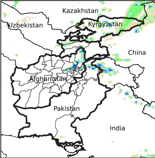
Daily Rainfall estimate for May 24, 2024
