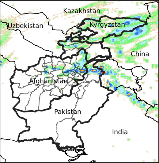
Daily Rainfall estimate for May 23, 2024
