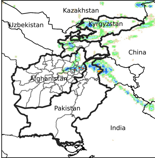
Daily Rainfall estimate for May 28, 2024
