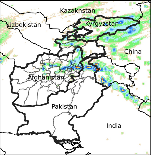
Daily Rainfall estimate for May 26, 2024
