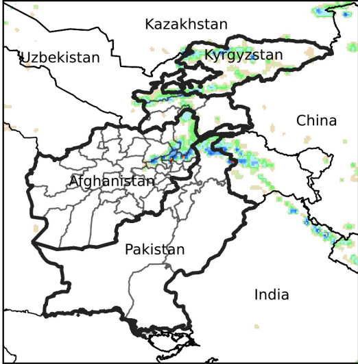
Daily Rainfall estimate for May 27, 2024
