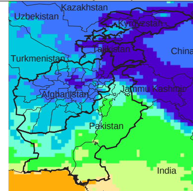
Mean Daily Temp. 2010
