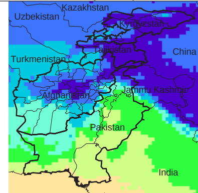
Mean Daily Temp. 2012
