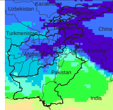
Mean Daily Temp. 2014
