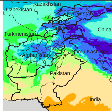
Mean Daily Temp. ('61-'90 avg)
