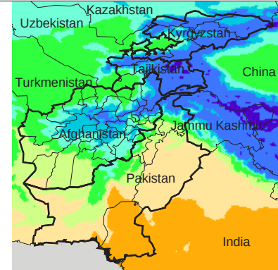
Mean Daily Temp. ('61-'90 avg)
