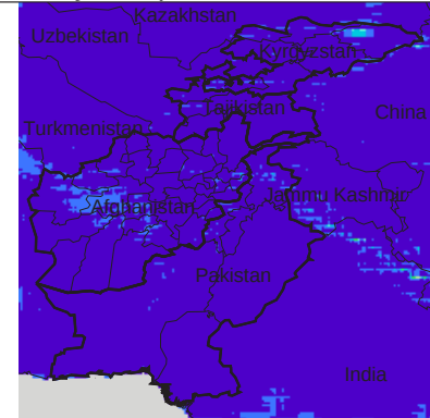
Mean Daily Temp. Difference from average
