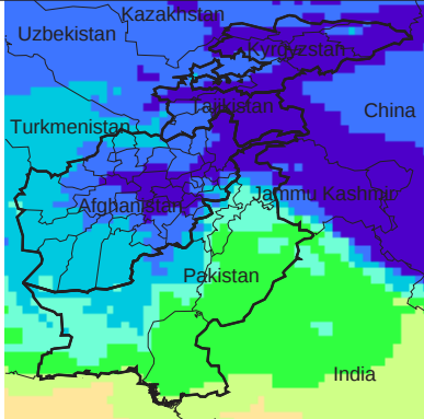
Mean Daily Temp. 2014
