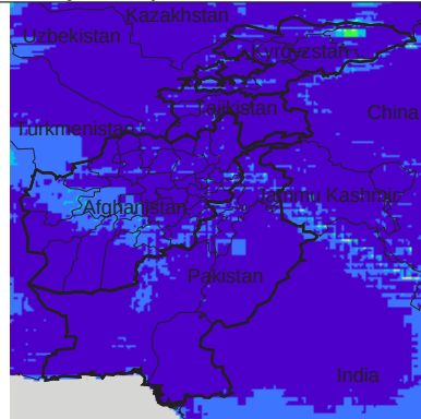
Mean Daily Temp. Difference from average
