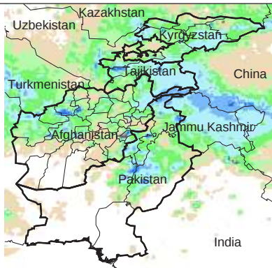
Total Dekadal Rainfall 2010
