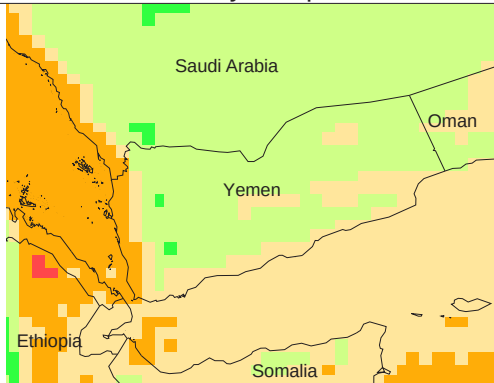
Mean Daily Temp. 2012
