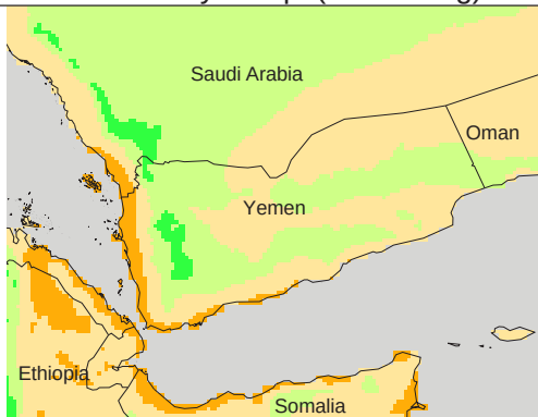
Mean Daily Temp. ('61-'90 avg)
