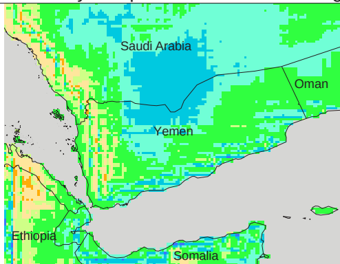
Mean Daily Temp. Difference from average
