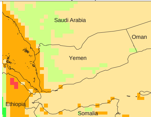
Mean Daily Temp. 2012
