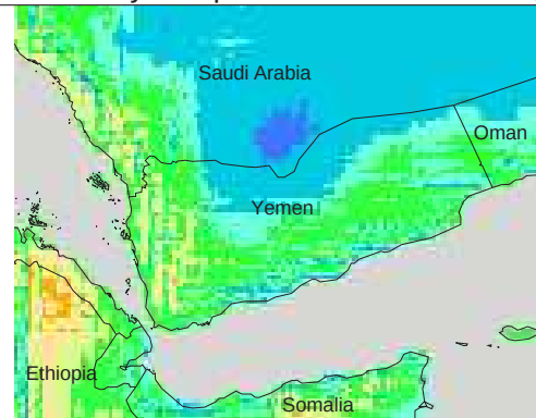
Mean Daily Temp. Difference from average
