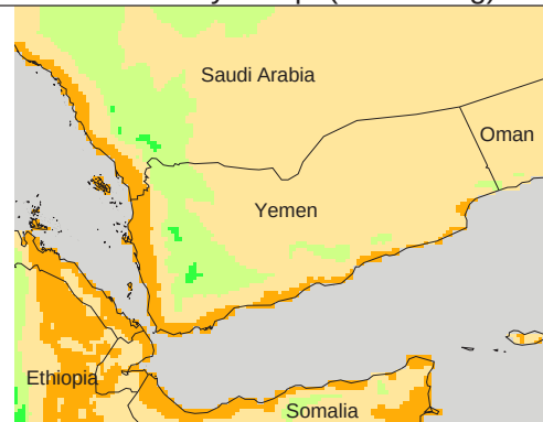
Mean Daily Temp. ('61-'90 avg)
