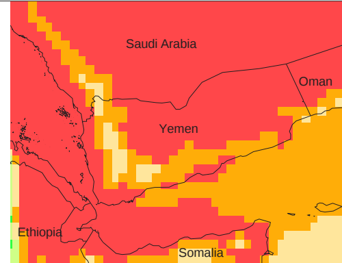
Mean Daily Temp. 2013
