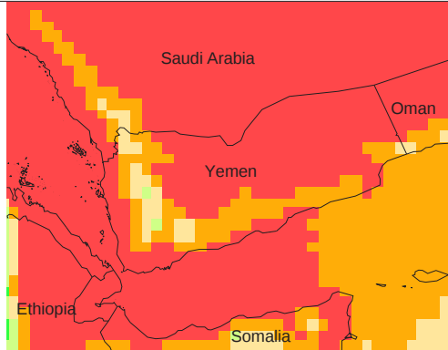
Mean Daily Temp. 2013
