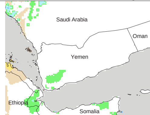
Dekadal Difference from average
