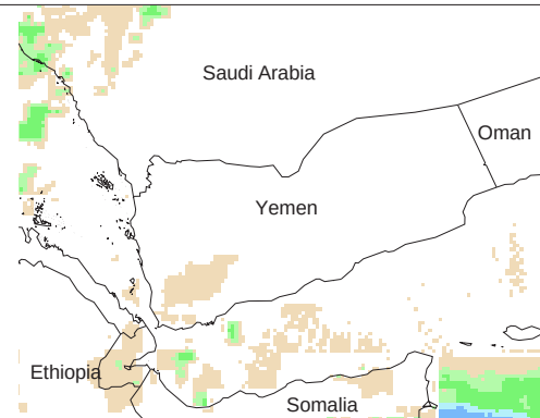
Total Dekadal Rainfall 2012
