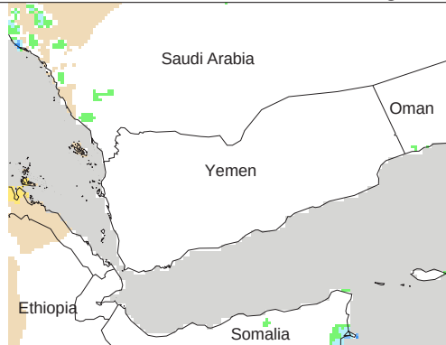
Dekadal Difference from average
